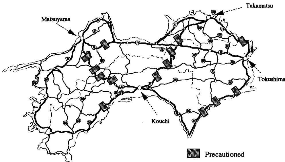
Figure 4 Location of Precautioned Sections of Shikoku Road Network (a quotation from reference 1)
